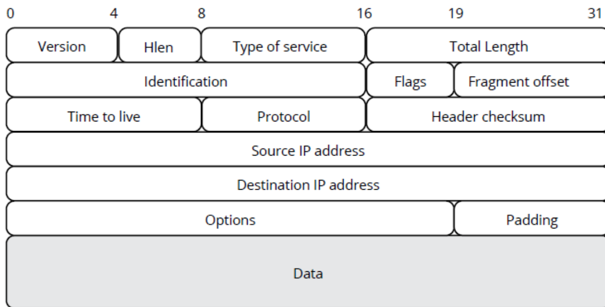
Figura: Layout do datagrama IP.
